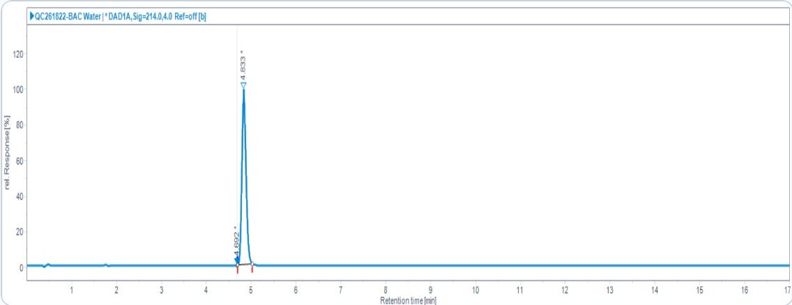
HPLC Chromatogram (Retention Time: 4.833 min)
